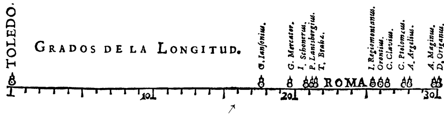
Figure 1.4. Langren's 1644 graph of determinations of the distance, in longitude, from Toledo to Rome. The correct distance is 16^{\circ}30' . Source: Tufté (1997, p. 15)
